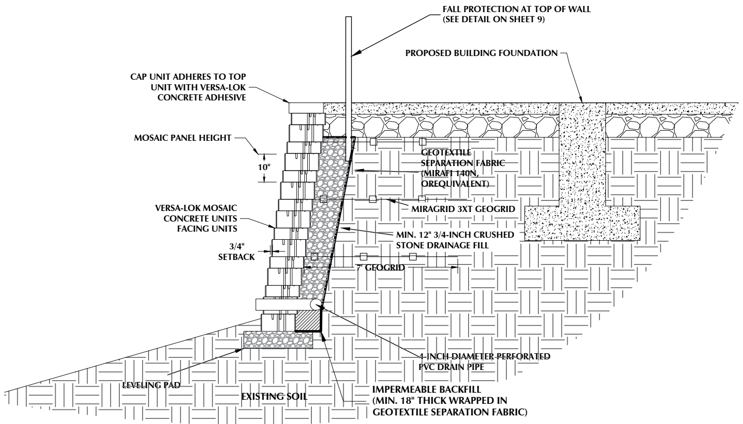
TYPICAL WALL SECTION - MSE BLOCK RETAINING WALL
