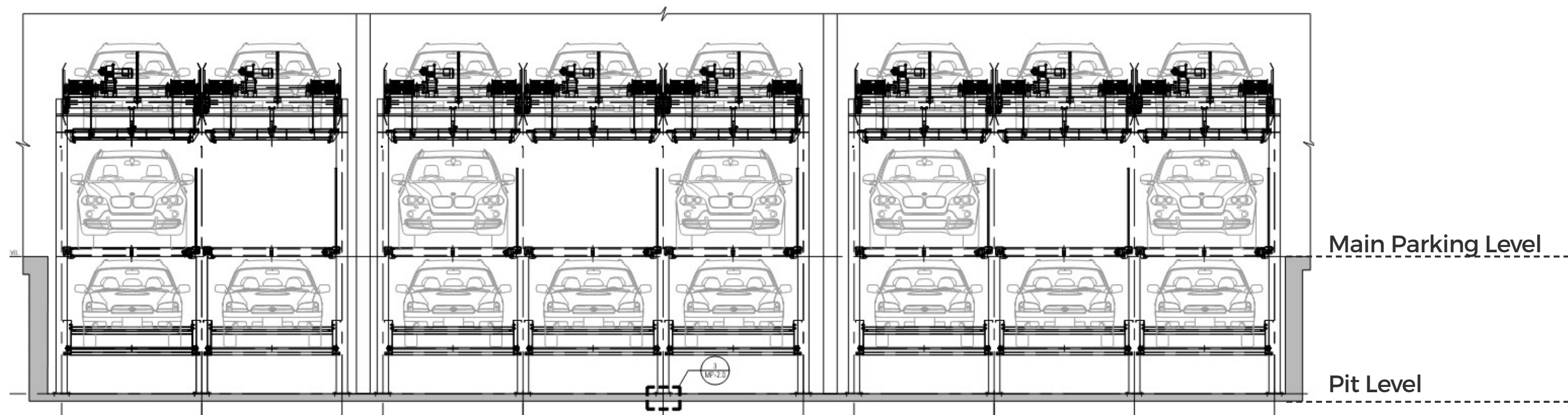
Conceptual Elevation
