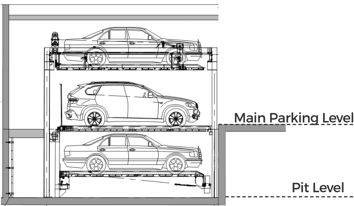
Conceptual Section
