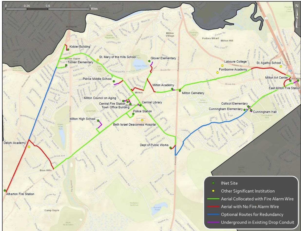
Figure 1: System-Level Fiber Network Architecture
